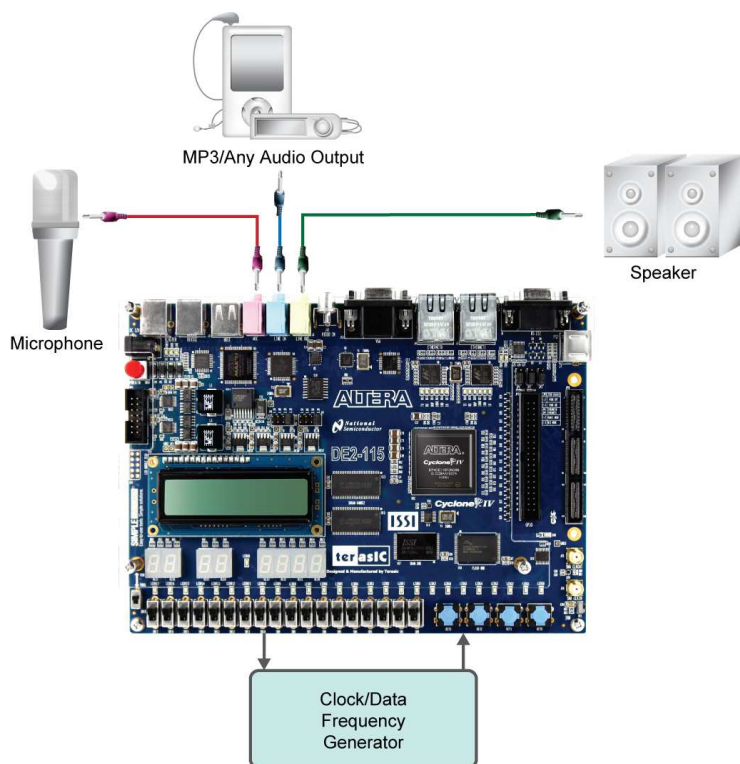
Figure 6-8 The setup for the Karaoke Machine
