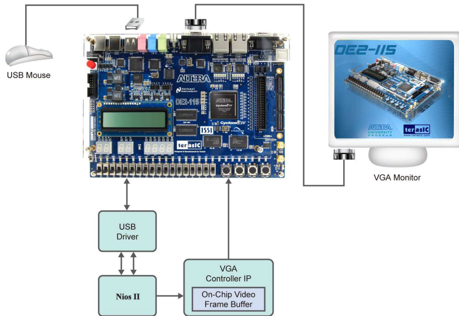
Figure 6-4 The setup for the USB paintbrush demonstration
