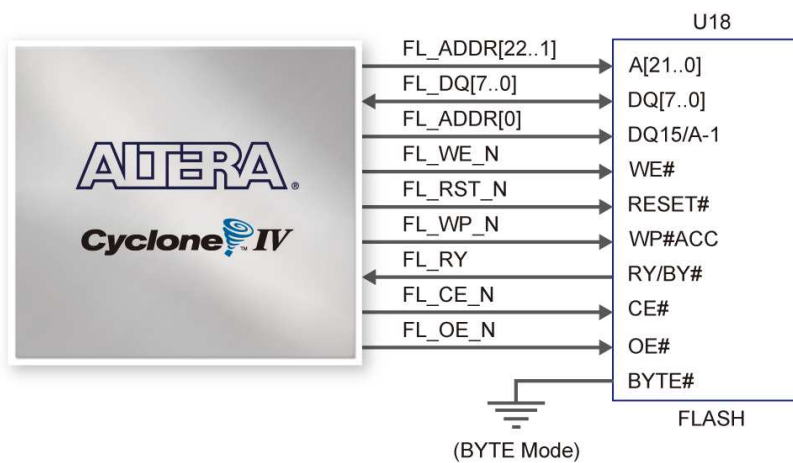
Figure 4-35 Connections between FPGA and Flash
