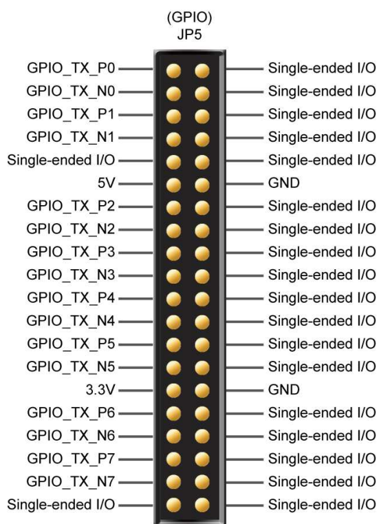
Figure 4-18 Pin defined when using LVDS interface on GPIO FPGA pins
