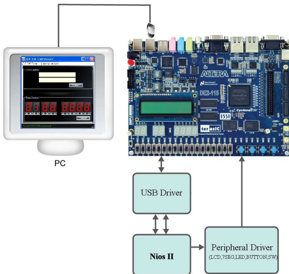
Figure 6-6 Setup for the USB device demonstration
